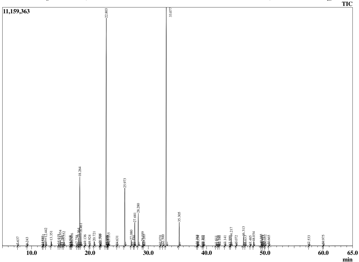
Chromatogram Lavandin, Australia C:\GCMSsolution\Data\EOU\EOU Donation\EOA Lavandin, Australia SRF17104.qgd
